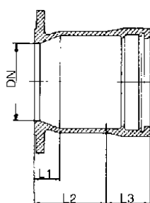
S-9170-4 Flanged socket PN 10
