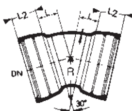
S-9175 Double socket bend 30°
