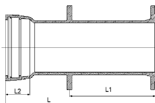
S-9173-14 Flanged socket With grouting collar
