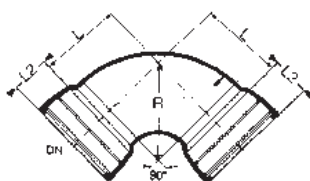
S-9175 Double socket bend 90°
