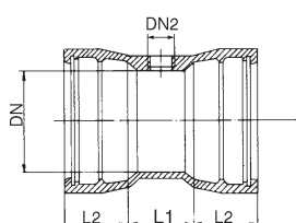
S-9171 Double socket With threaded branch
